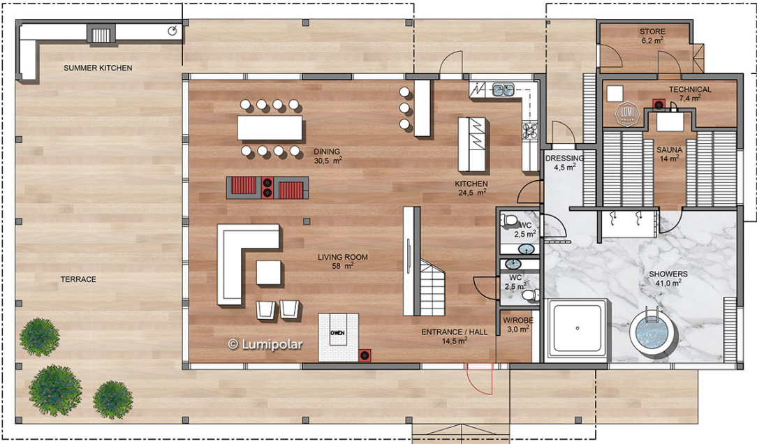
1 Floor
