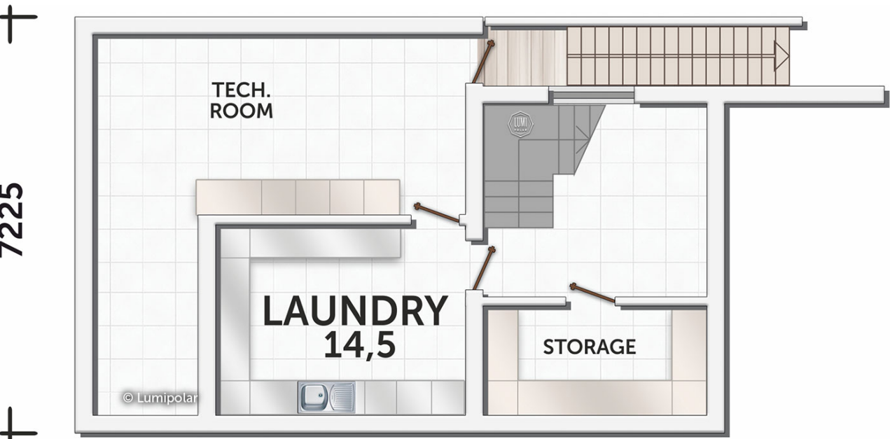
Basement
